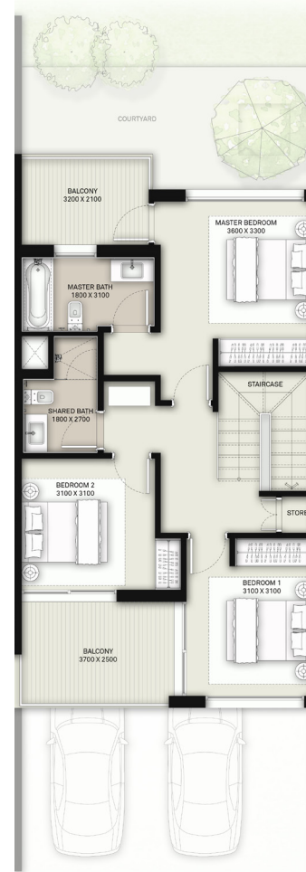
FIRST FLOOR
