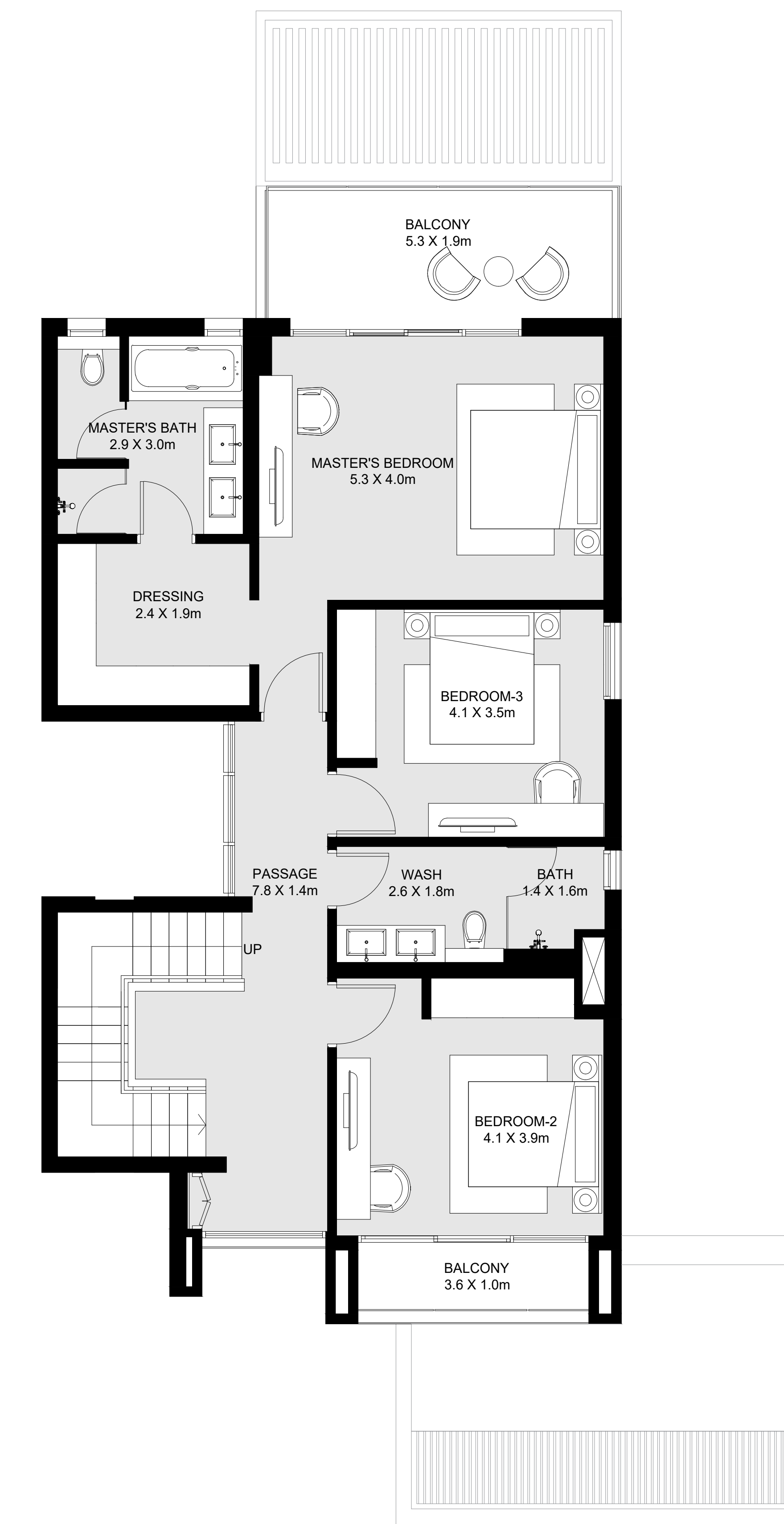
FIRST FLOOR
