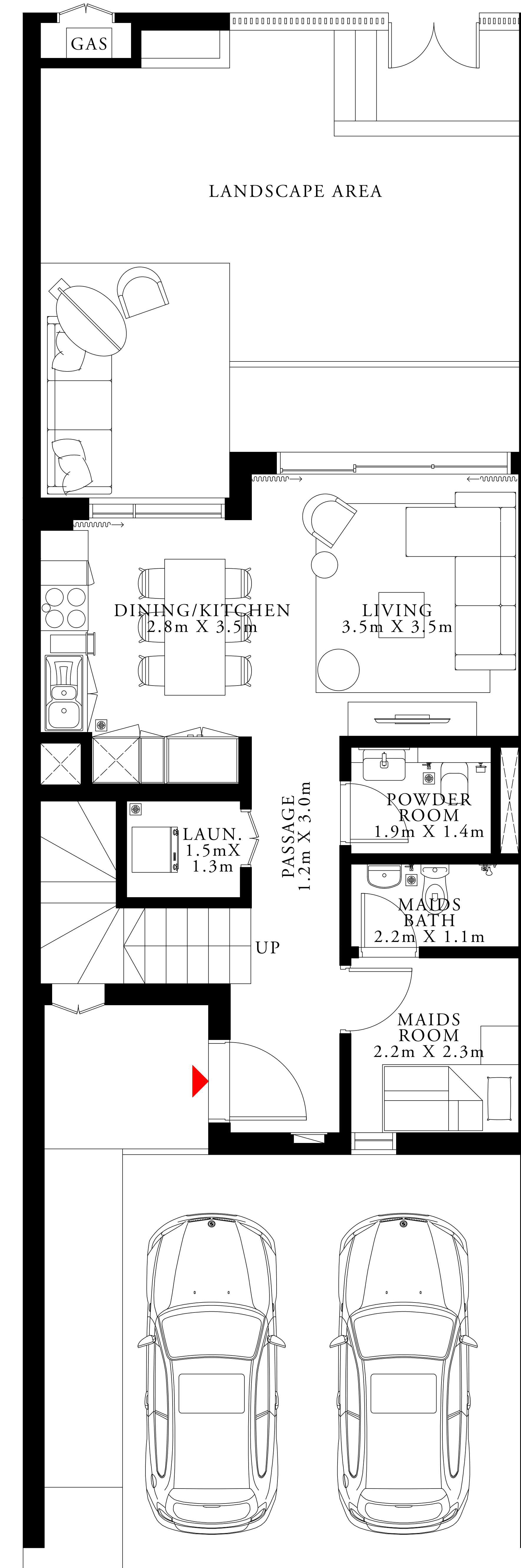
GROUND FLOOR
